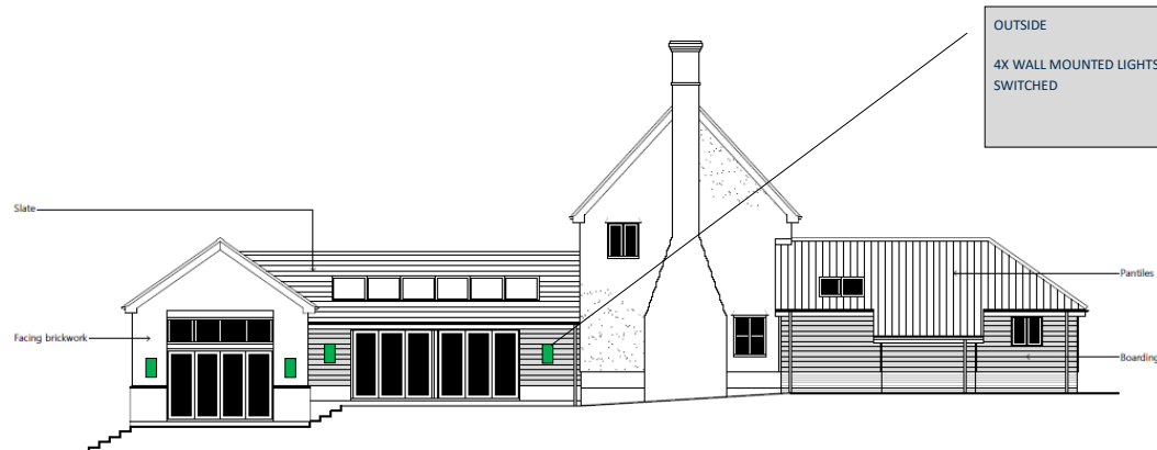
Proposed side (north-east) elevation 1:100
